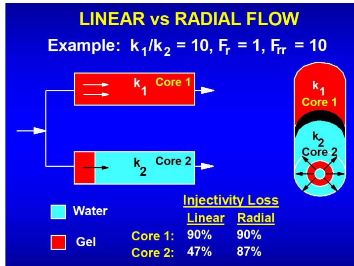
Figure 1.15. Theoretical comparison of permeability reduction in linear versus radial flow.
