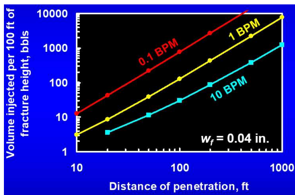
Figure 1.23. Predicted gel propagation through a two-wing 1-mm-wide vertical fracture.
