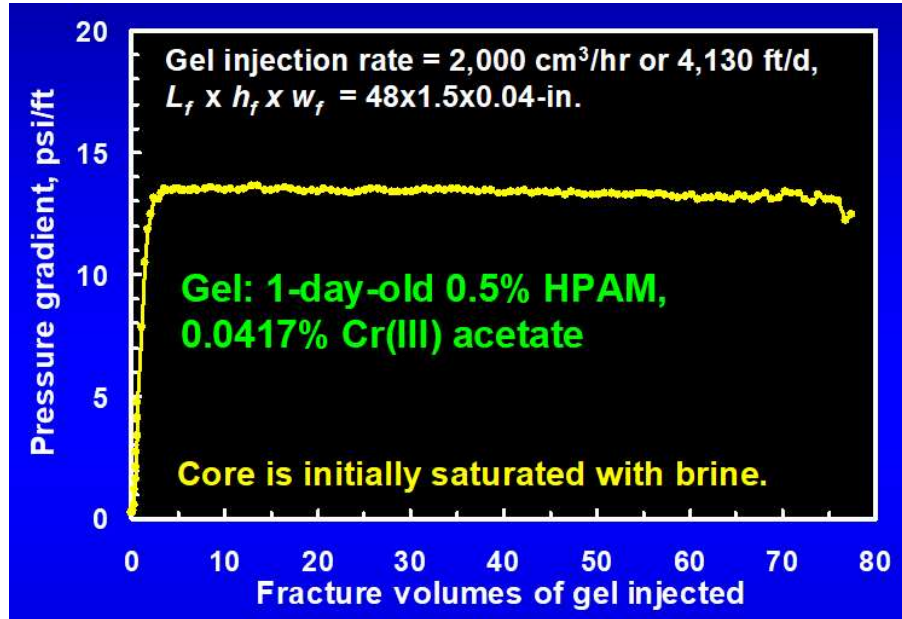
Figure 1.17. Stable extrusion of a Cr(III)-acetate gel through a fracture.
