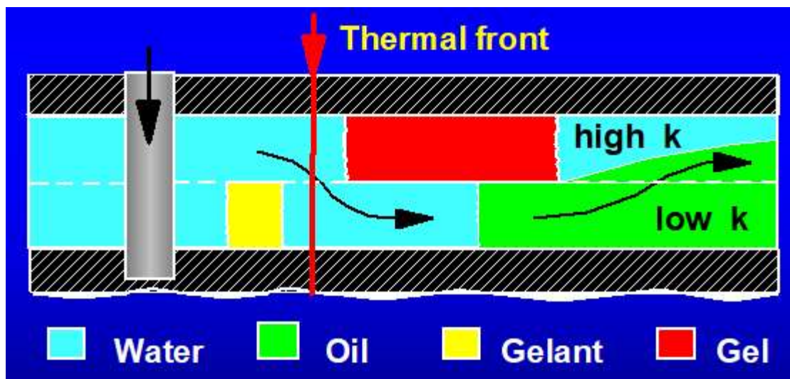
Figure 1.13. Illustration of in-depth profile modification.
