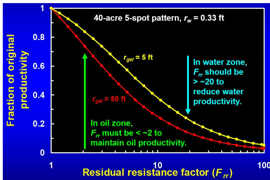
Figure 1.14. Permeability reduction requirements for treatment of unfractured vertical wells without zone isolation.
