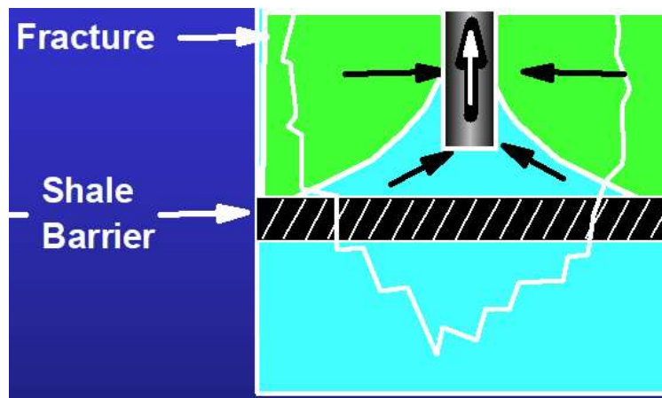
Figure 1.7. Fracture leading from a vertical production well down to an aquifer.
