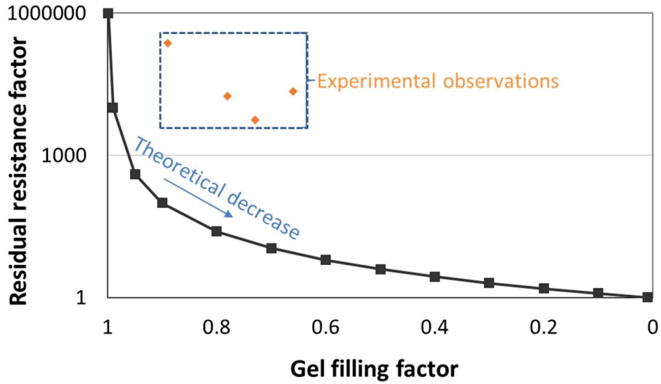
Figure 1.26: Calculated residual resistance factor for a fracture initially filled with concentrated gel, using the cubic law k_f = \frac{\text{fracture width}^2}{12} [187]. Gel washes out of the middle of the fracture first according to the Carter model, and fracture conductivity is determined by the width of the active flow path. Experimental observations [188] do not corroborate the quickly decreasing gel permeability reduction.
