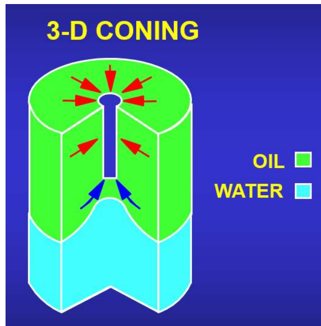
Figure 1.10. 3D coning from an underlying aquifer (no fractures and no barriers to flow).
