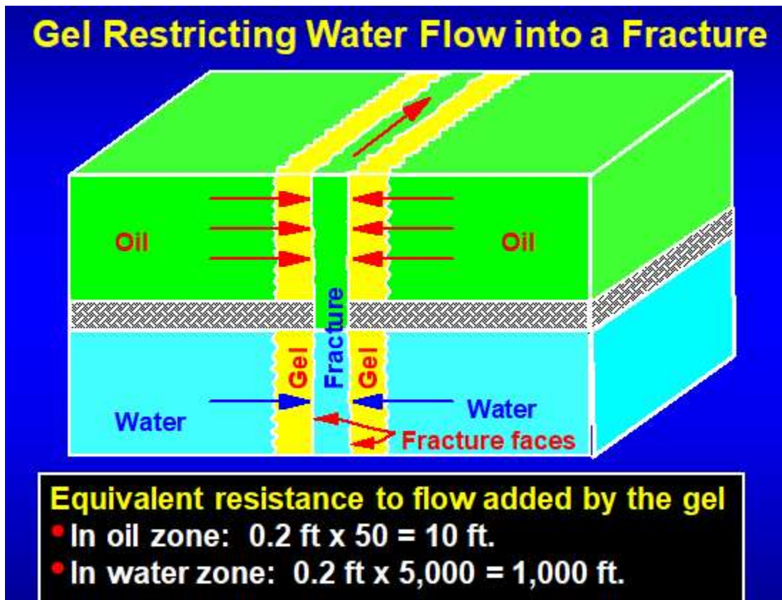
Figure 1.16. Gelant treatments of fractured production wells.
