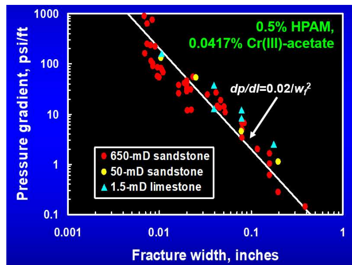
Figure 1.18. Pressure gradient for gel extrusion versus fracture width.
