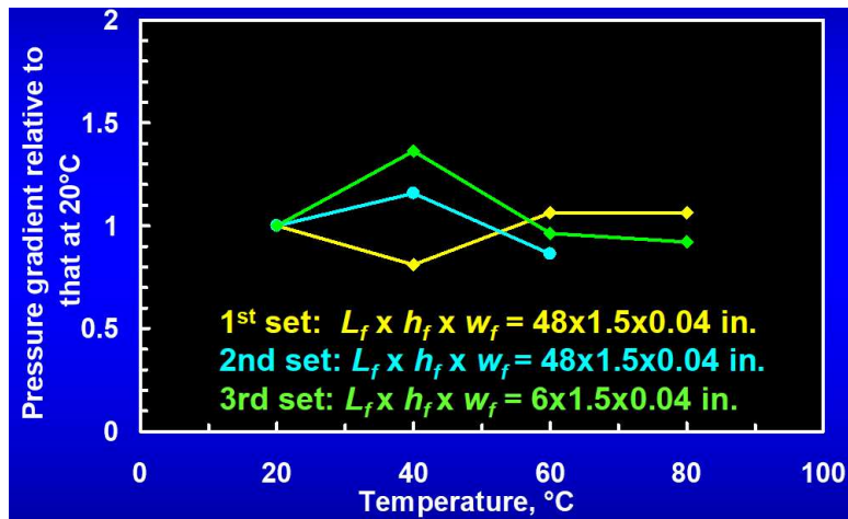
Figure 1.20. Pressure gradient for gel extrusion versus temperature.
