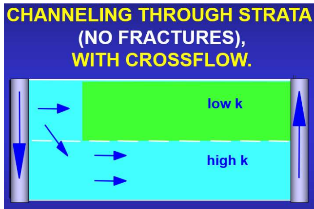
Figure 1.12. Channeling from a nearby injection well (no fractures and no barriers to flow).
