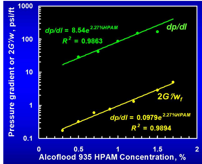
Figure 1.19. Pressure gradient for gel extrusion versus polymer concentration.
