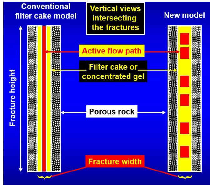
Figure 1.24. Old Carter model versus new gel-extrusion model.
