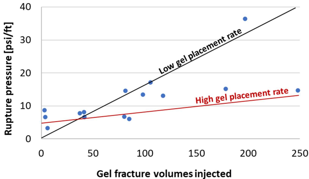
Figure 1.25: Dehydrated gel can withstand higher pressure gradients during subsequent chase floods. Gel dehydration within a specific segment of the fracture is maximized by injecting more gel or using lower injection rates.
