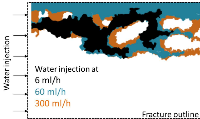
Figure 1.28: wormhole development within a 1-mm wide fracture captured by PET imaging. Injected water was labelled with positron-emitting isotope ^{18}\text{F} -FDG. Upon combinations between emitted positrons and adjacent electrons, a photon pair with 511keV energy is emitted, and this event can be spatially and temporally determined. Details are provided in [188].
