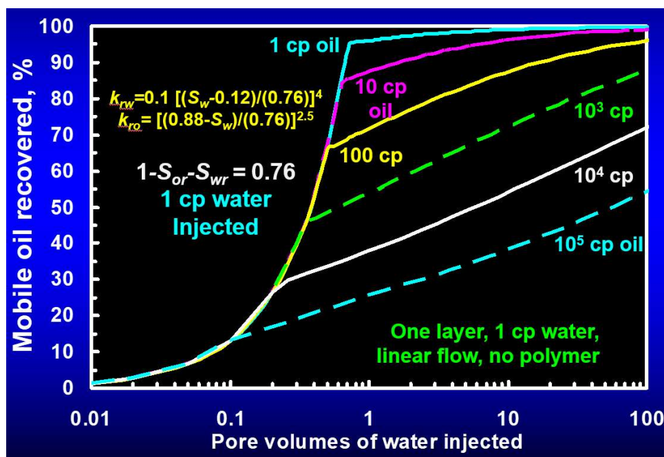
Figure 1.1. Expected oil recovery vs PV water injected.
