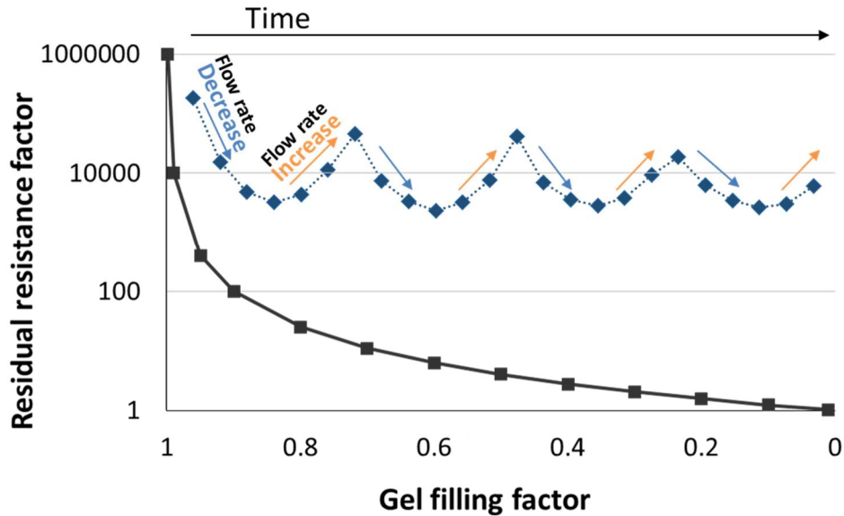
Figure 1.27: Permeability reduction provided by gel remains high over time and vary with injection rate and pressure. Full data set available in [185].
