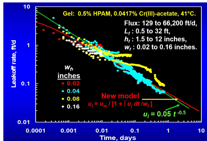
Figure 1.22. Leakoff rates during gel extrusion through fractures.
