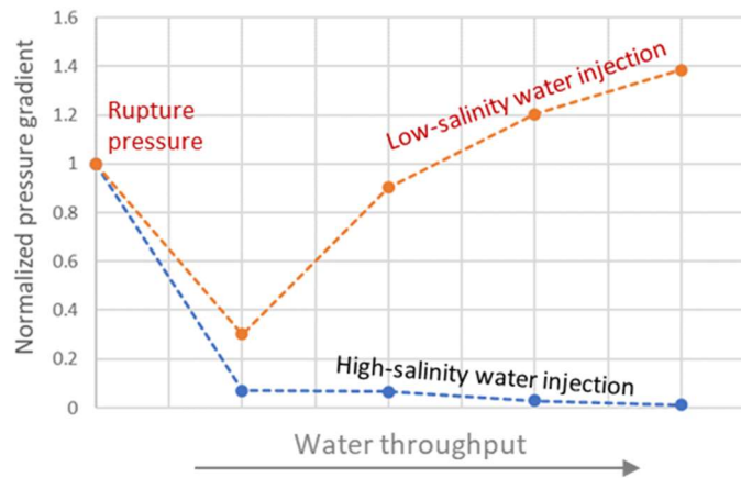
Figure 1.30: Water may flow through the fracture after gel rupture. When there is no salinity contrast between the gel and injected water, the permeability reduction provided by gel will decrease with water throughput. The opposite trend is observed when the salinity in the injected water phase is decreased compared to the gel and the permeability reduction provided by gel increased with time.
