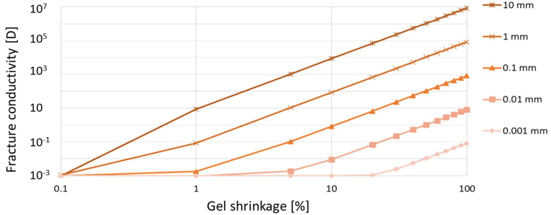
Figure 1.29: shrinkage of gel and its influence on fracture conductivity for different fracture widths. The fracture is assumed to be filled by concentrated gel initially.
