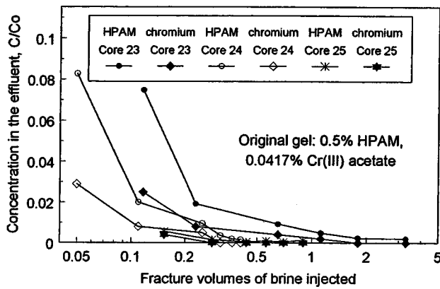
Fig. 8—Chromium and HPAM concentrations produced from cores 23, 24, and 25 during brine injection after gel placement.
