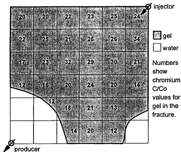
Fig. 11—Relative chromium concentrations in horizontal fracture 1 (12 in. × 12 in. × ~0.01 in.) after gel placement.
