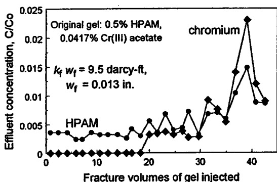
Fig. 1—Chromium and HPAM effluent concentrations during gel injection into core 15 (relative to injected concentrations).
