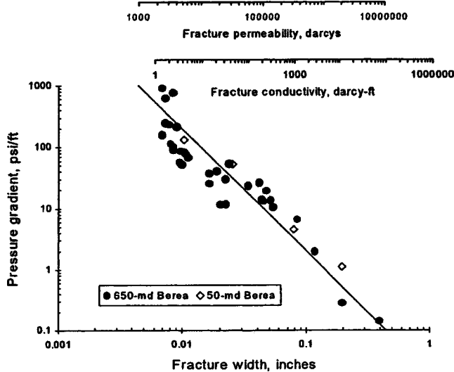
Fig. 6—Pressure gradients during extrusion of a 1-day-old Cr(III)-acetate-HPAM gel using a fixed volumetric injection rate (12.2 in. 3 /h or 200 cm 3 /h).
