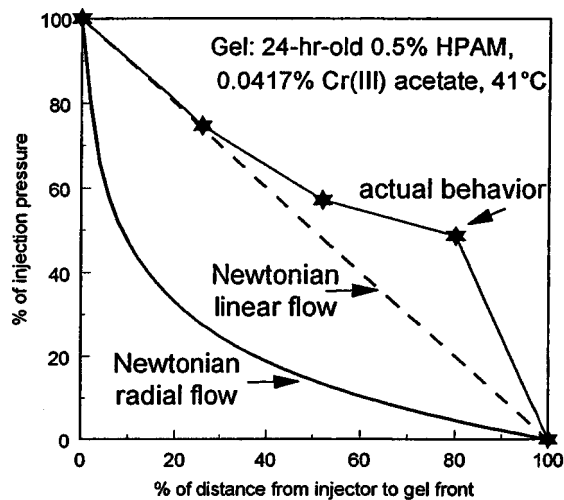
Fig. 10—Pressure behavior observed during gel injection into horizontal fracture 1.
