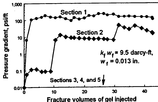
Fig. 2—Pressure gradients during gel injection into core 15.
