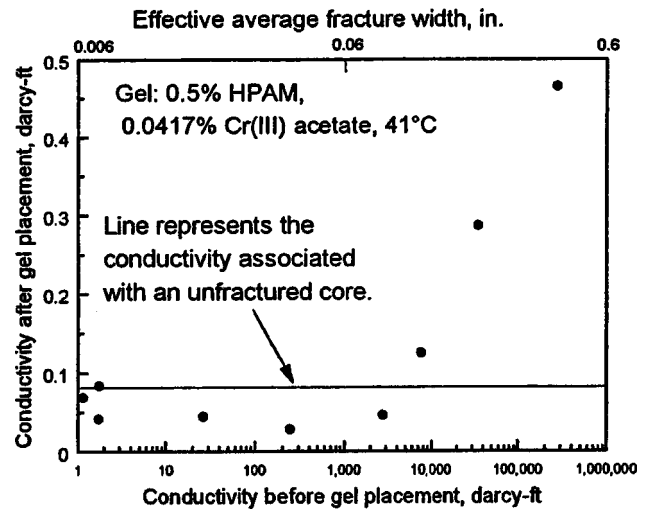
Fig. 7—Core conductivity during brine injection after gel placement vs fracture conductivity before gel placement.
