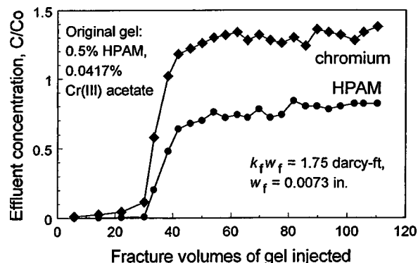
Fig. 5—Chromium and HPAM effluent concentrations during gel injection into core 20 (relative to injected concentrations).
