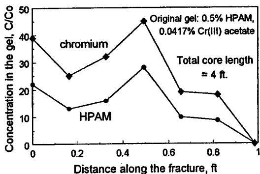
Fig. 3—Chromium and HPAM concentrations for gel in the fracture of core 15 (relative to injected concentrations).
