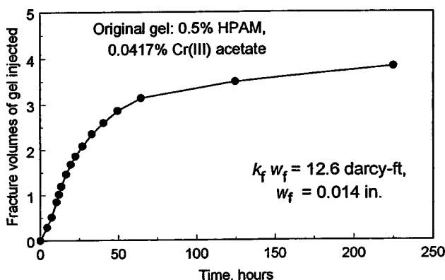
Fig. 4—Apparent gel extrusion with a constant pressure drop of 35 psi across a 4-ft-long core (core 16).
